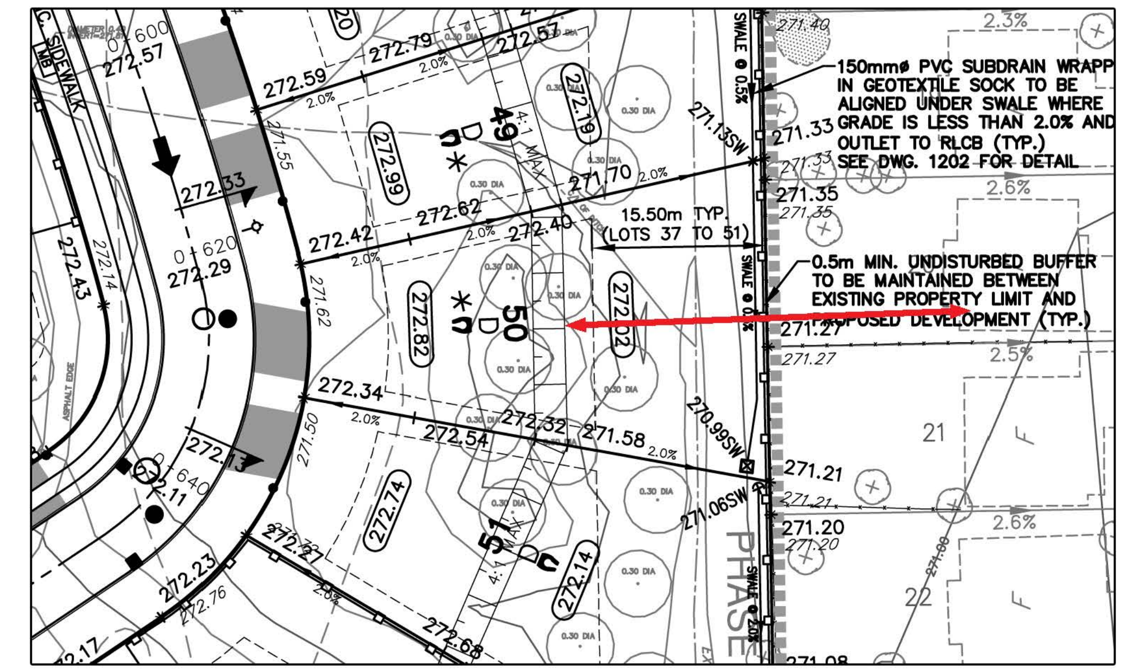
Grading Plan Excerpt - Lot 50
